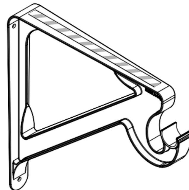
Shelf Bracket with Open Slide Rod For 12" Deep Shelves. Available in White and Nickel.
